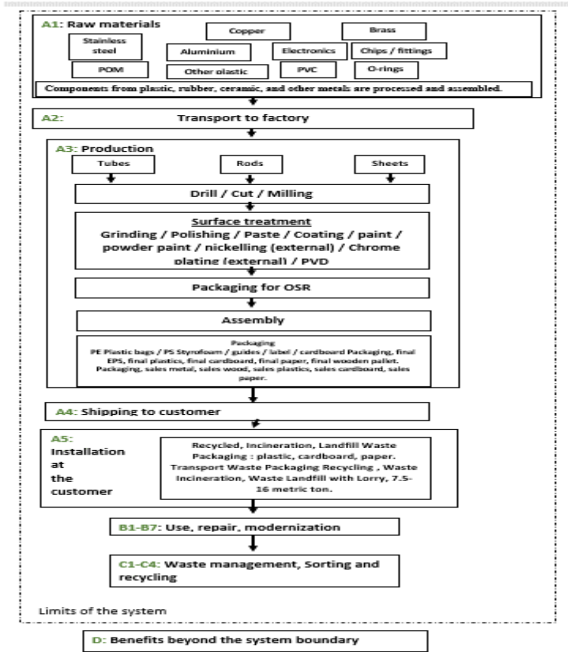
Figure 3: Flow diagram of product system with modules A1-D
